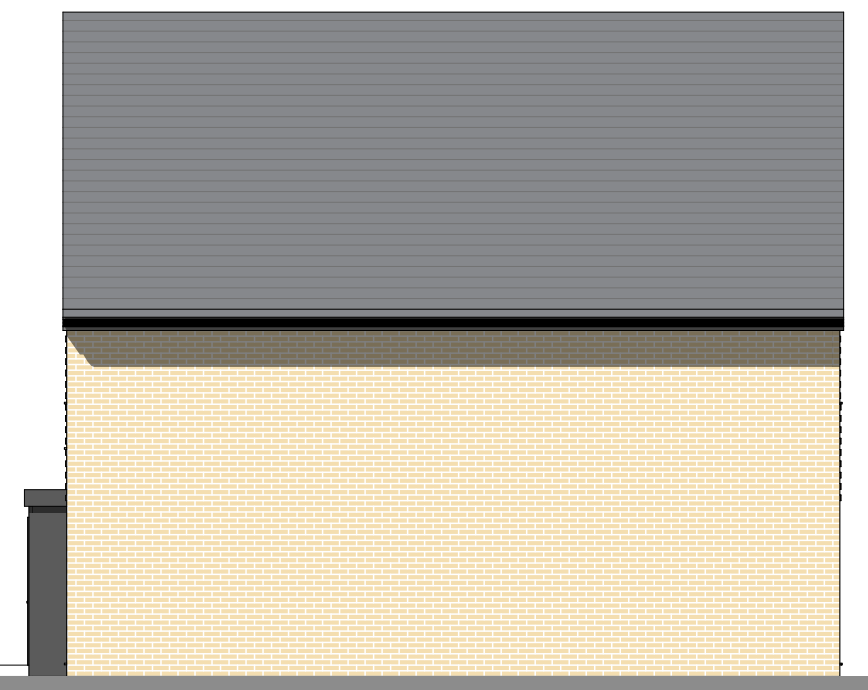
Side 2 Elevation 1:100
