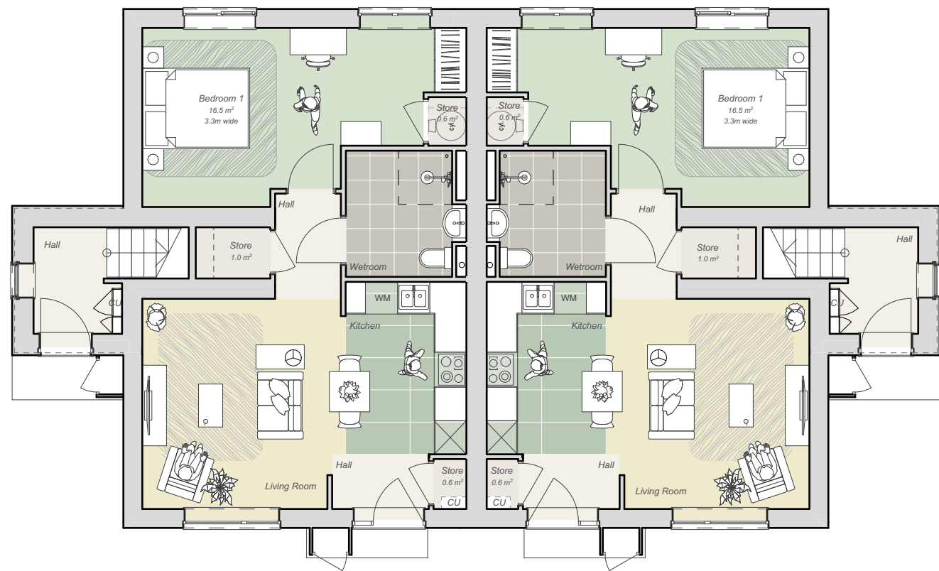
Ground Floor 1:100
