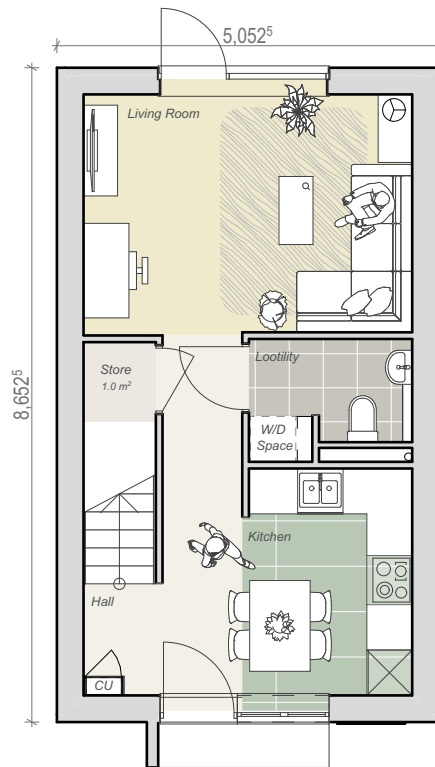
Ground Floor 1:100
