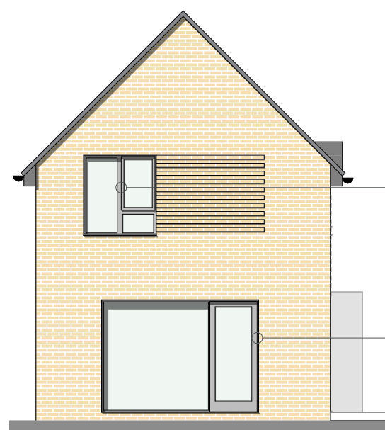
Rear Elevation 1:100
