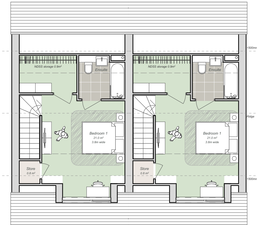
Second Floor 1:100
