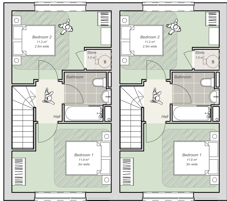
First Floor 1:100
