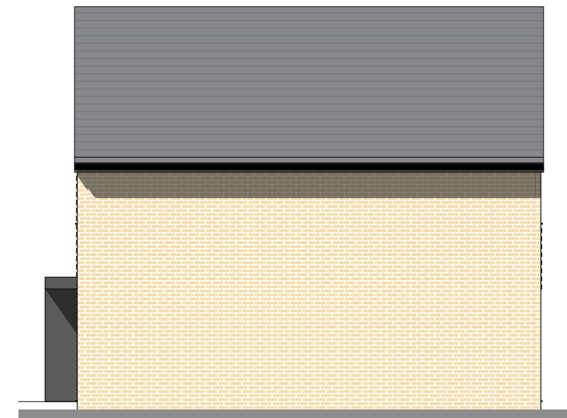
Side 2 Elevation 1:100
