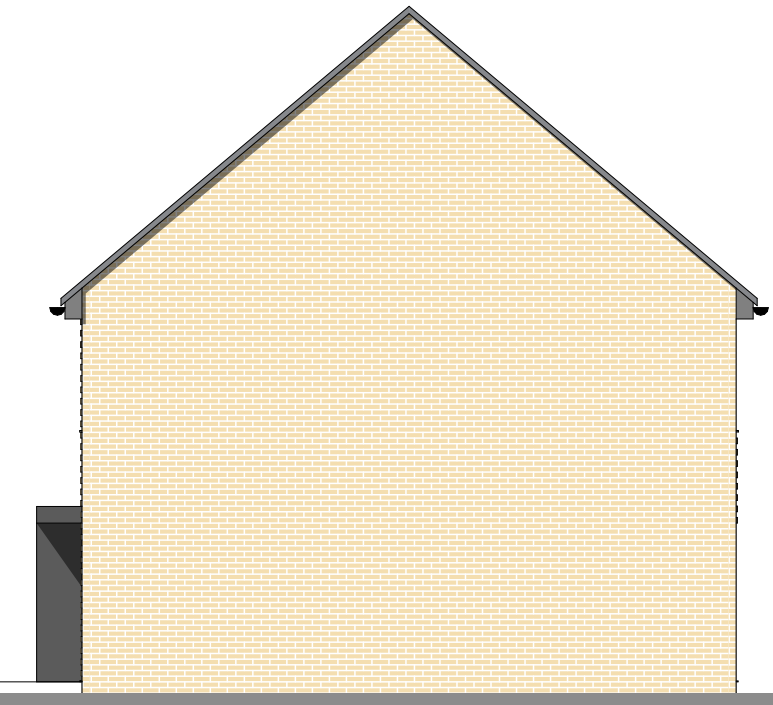
Side 2 Elevation 1:100
