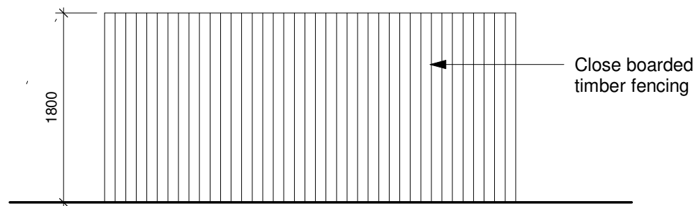
Timber Bin Enclosure Elevation 1 : 50
