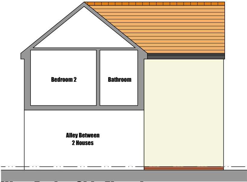
West Facing Side Elevation
