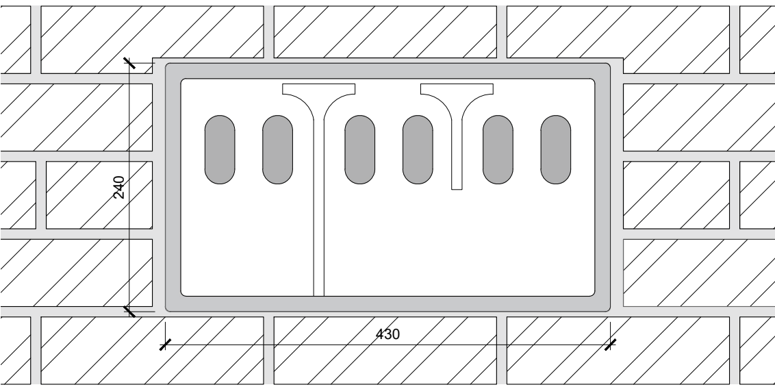
EXTERNAL WALL - BIRD NEST ELEVATION SCALE 1:5
