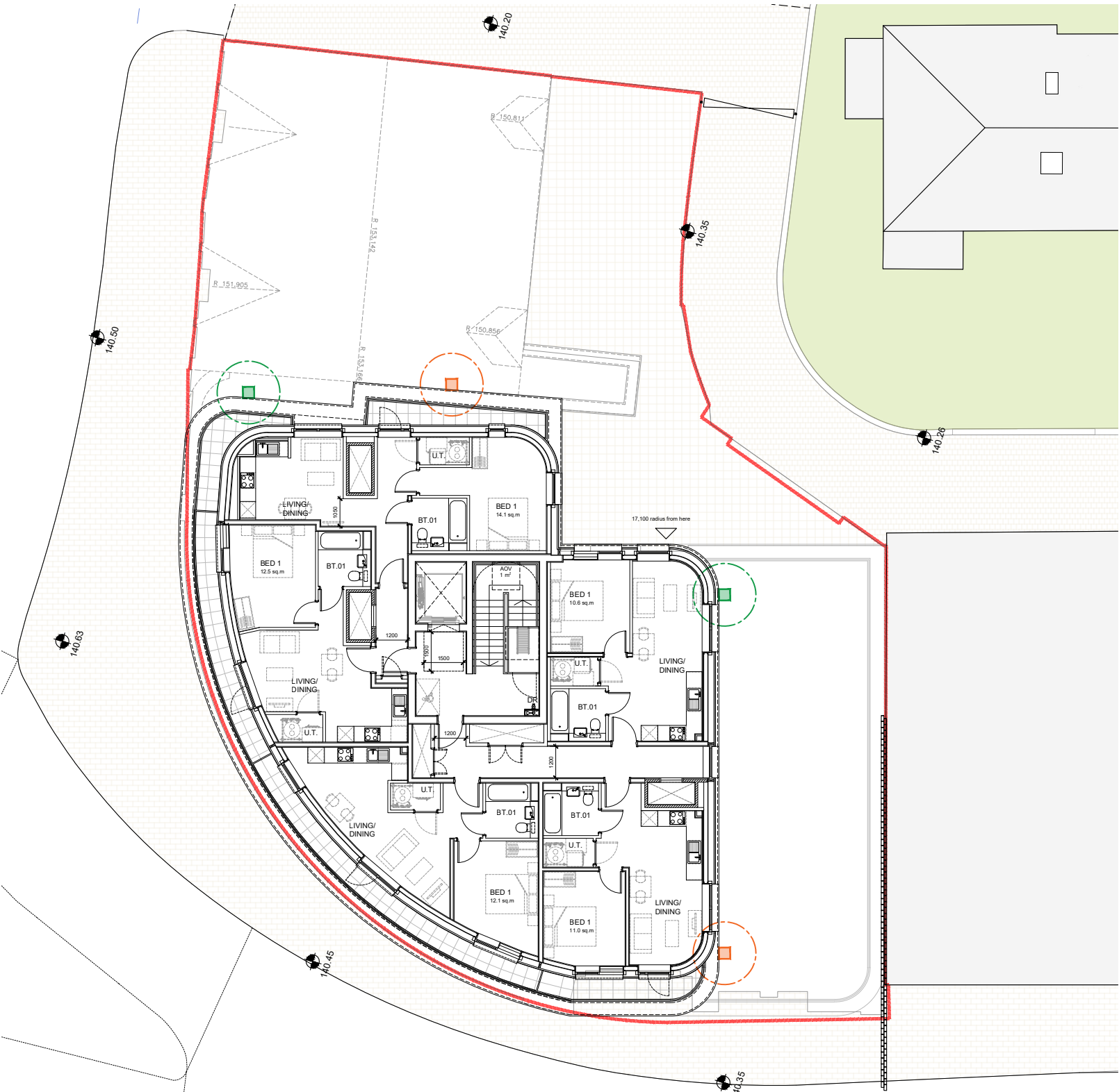
LOCATION + LEVEL 5 PLAN 1:200 SCALE
