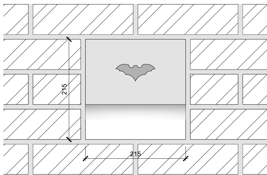
EXTERNAL WALL - BAT BOX ELEVATION SCALE 1:5
