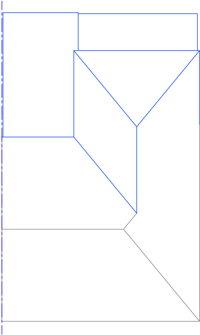
PROPOSED ROOF 1:100
