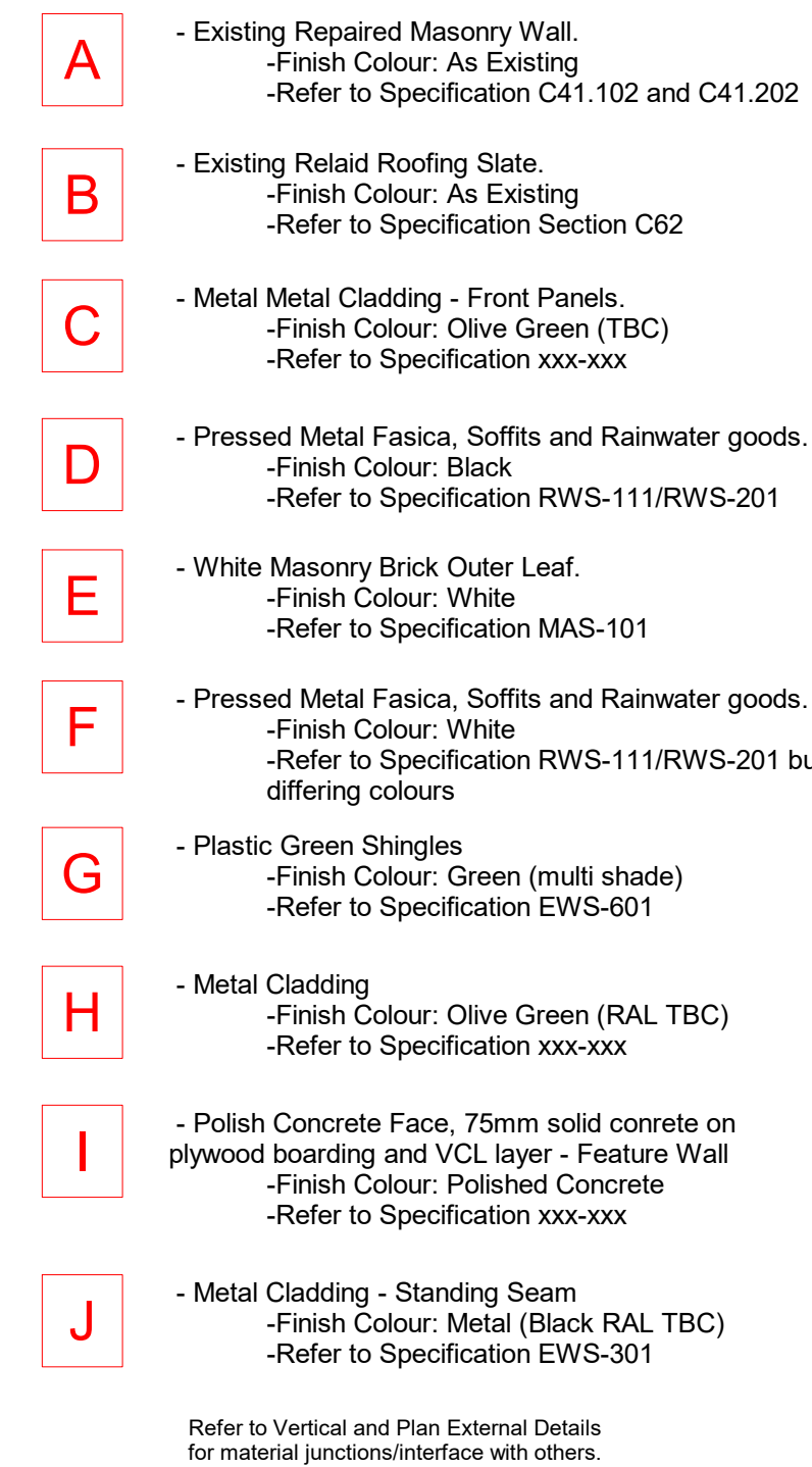
Elevation Materials Legend
