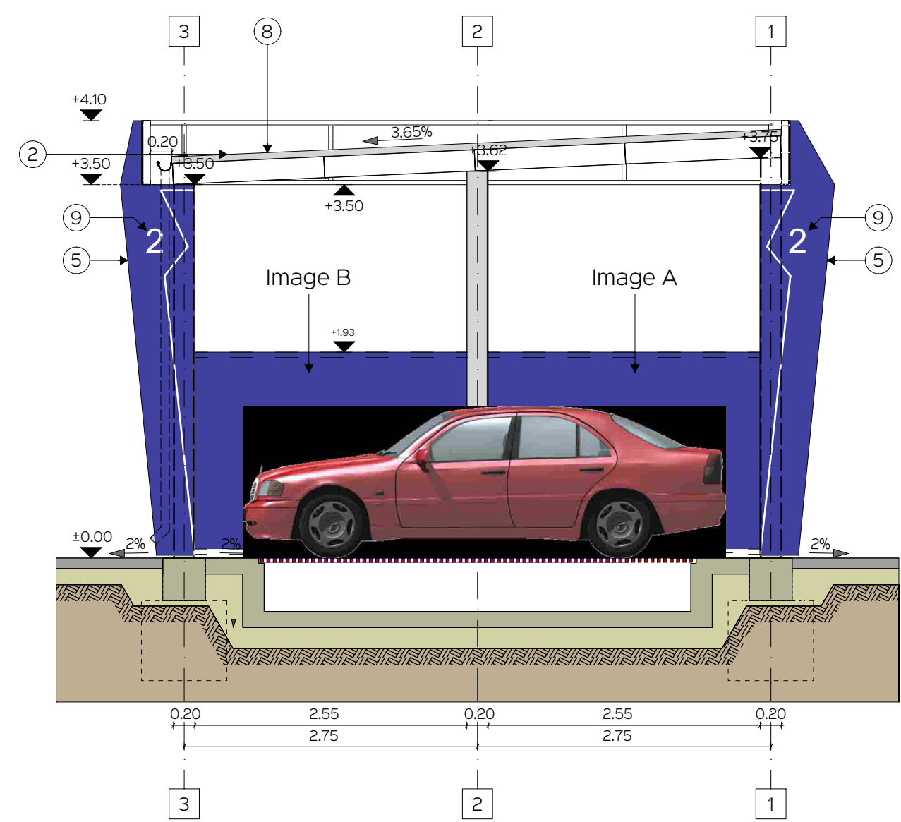
Short Section A - A (scale 1:50)
