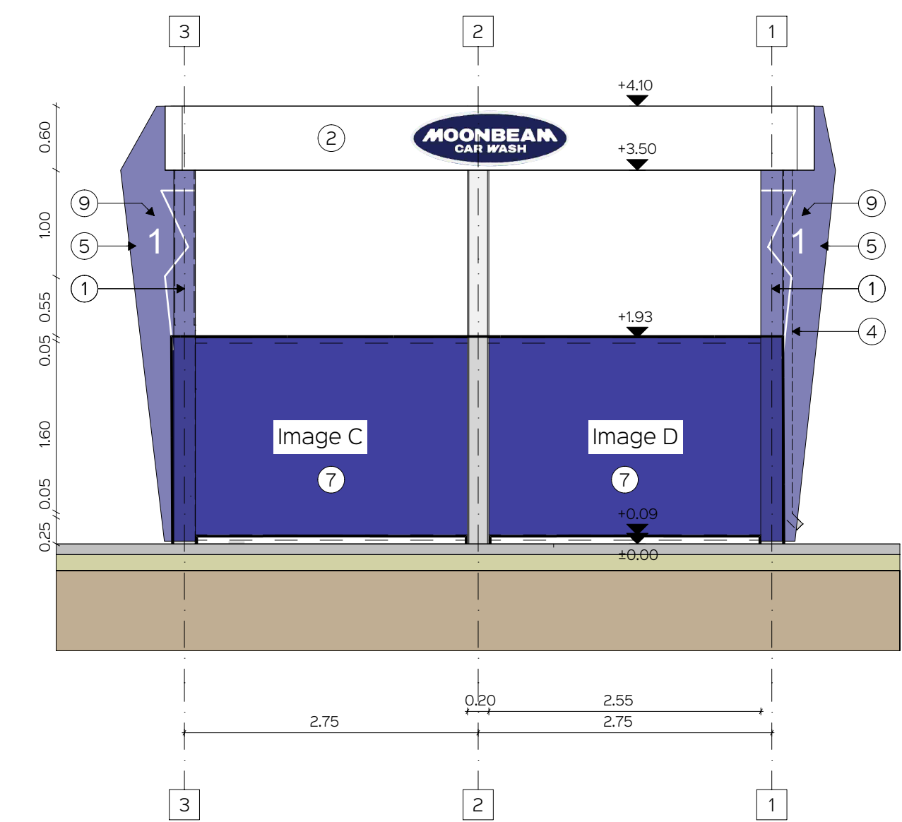
North West Side Elevation A (scale 1:50)
