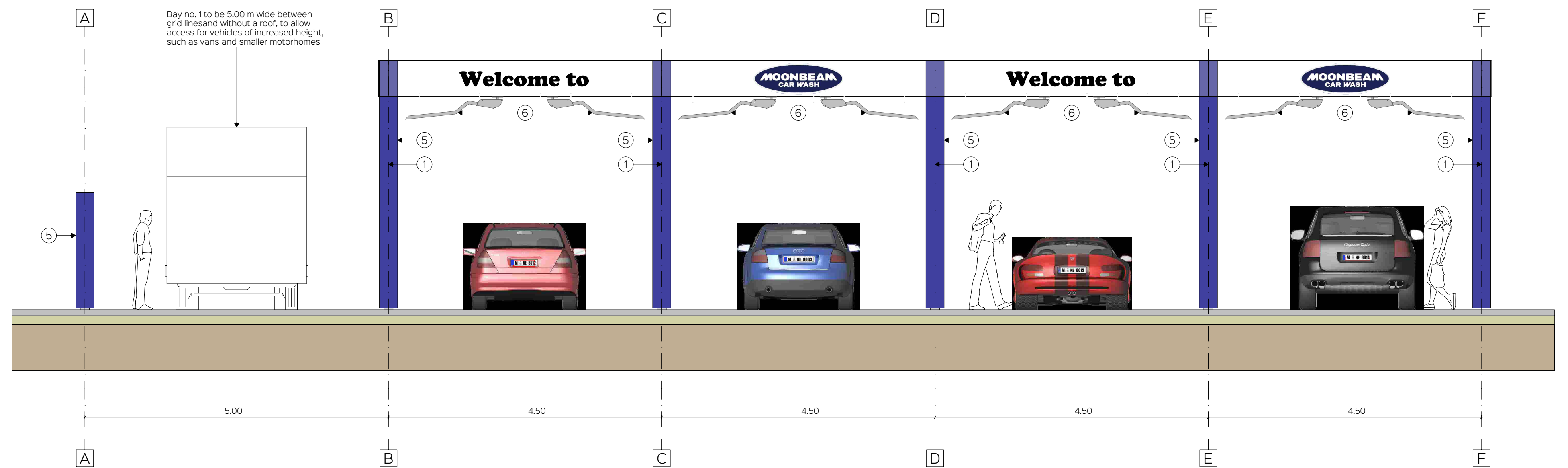
Front / South West (Entrance) Elevation (scale 1:50)
