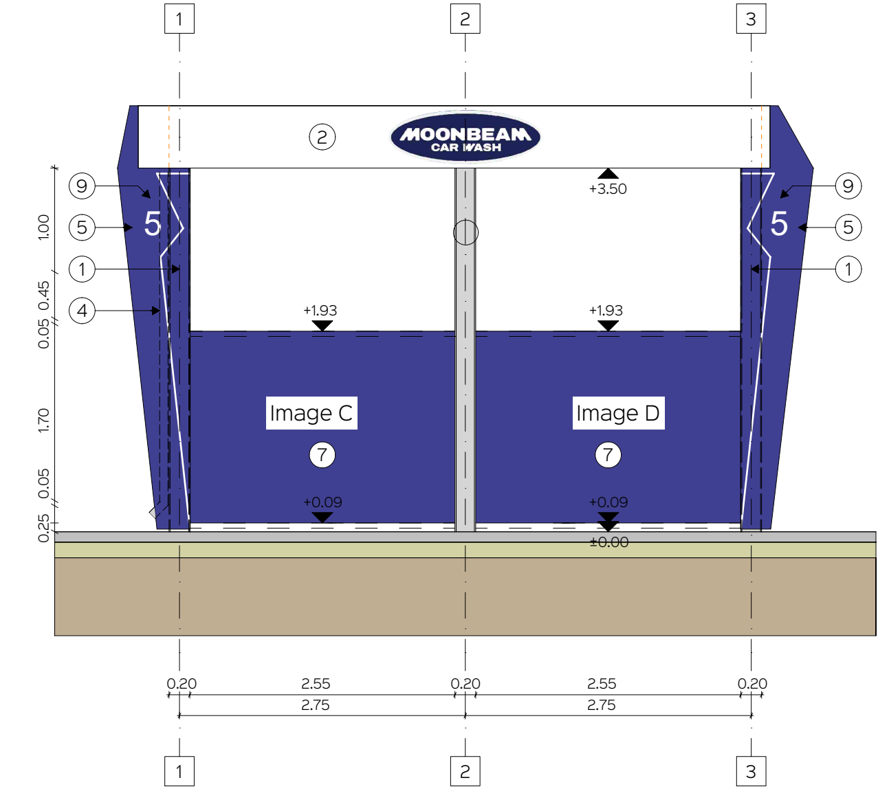
South East Side Elevation B Facing the Highway (scale 1:50)
