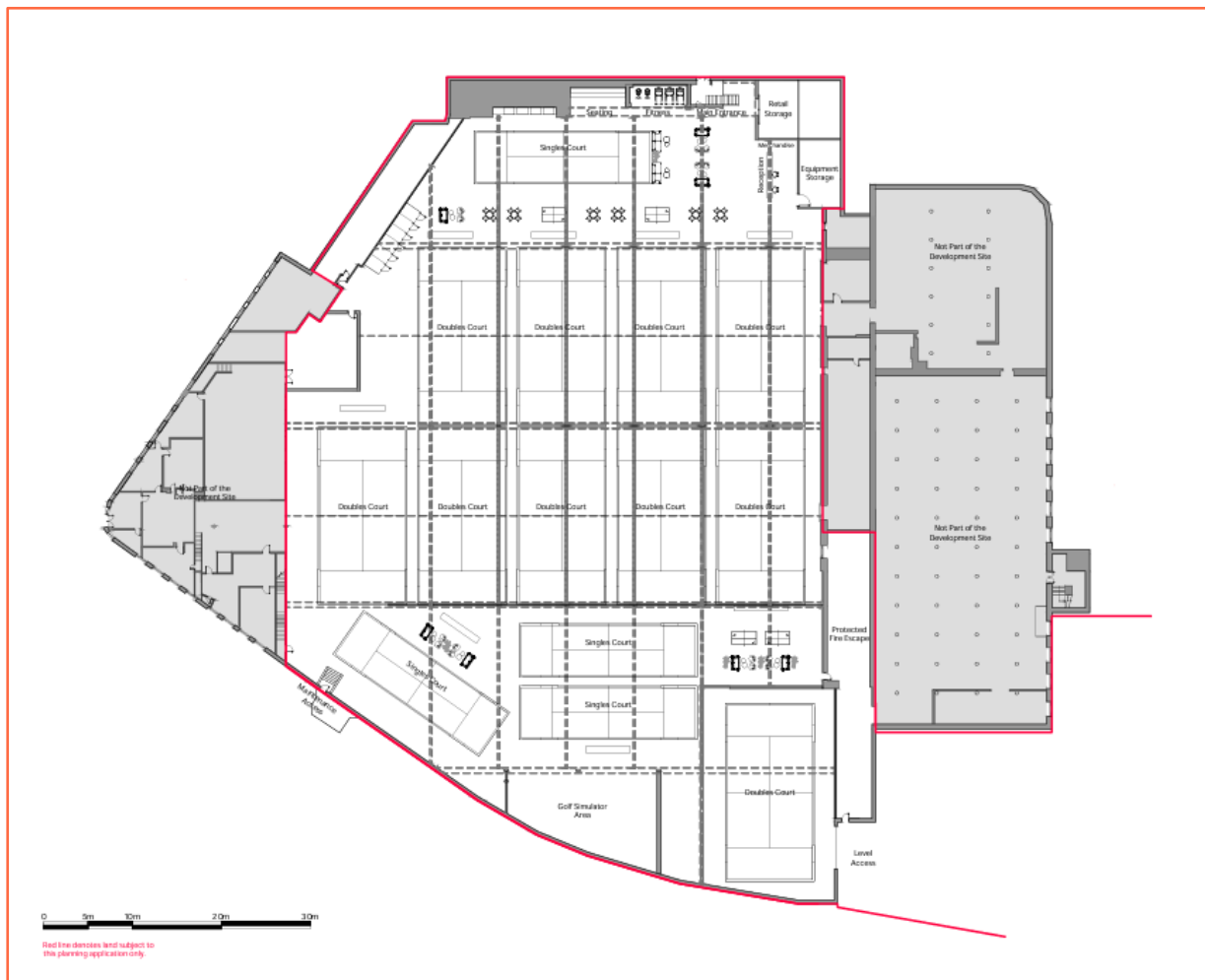
Figure 3: Proposed ground floor plan (Source: NC Studio)
