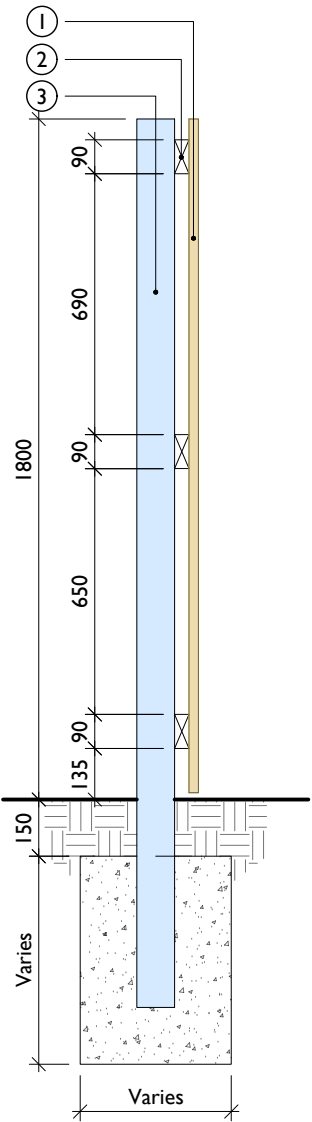
Section
