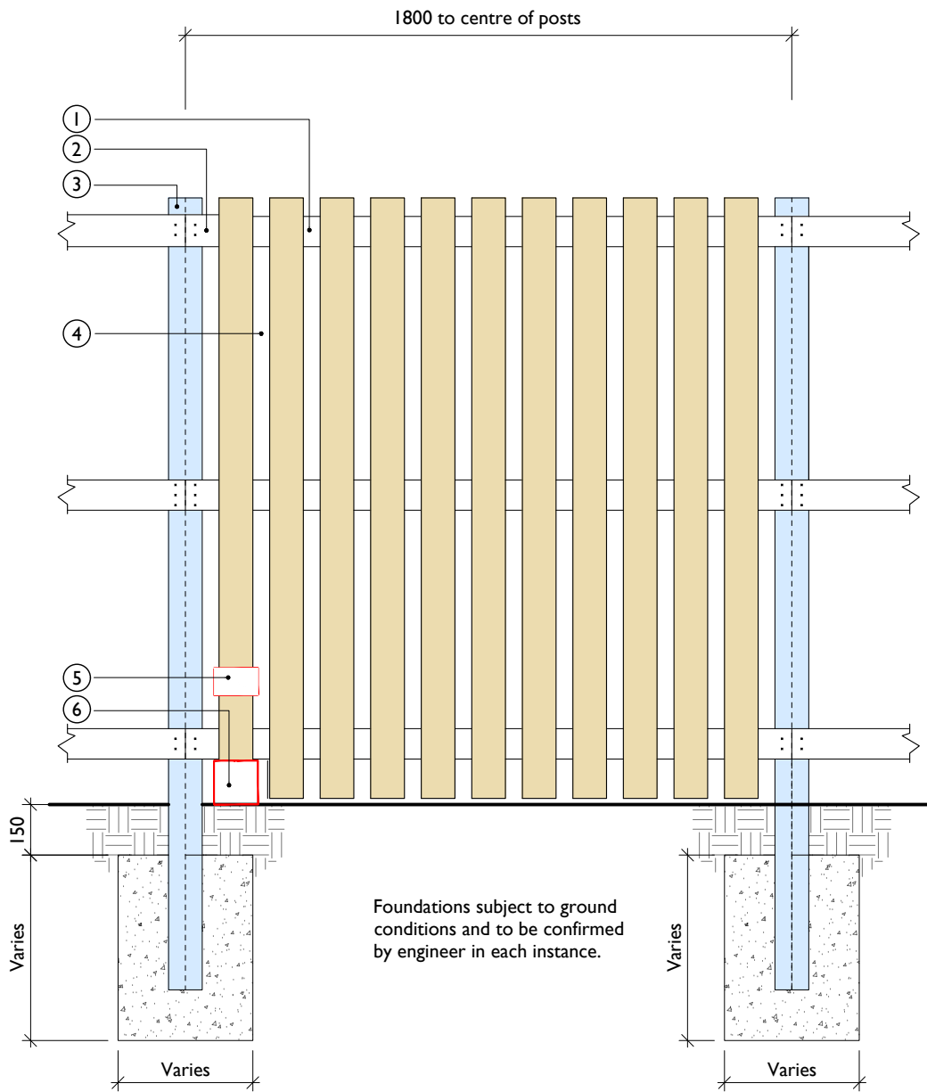
1.8m Hit and miss fence
