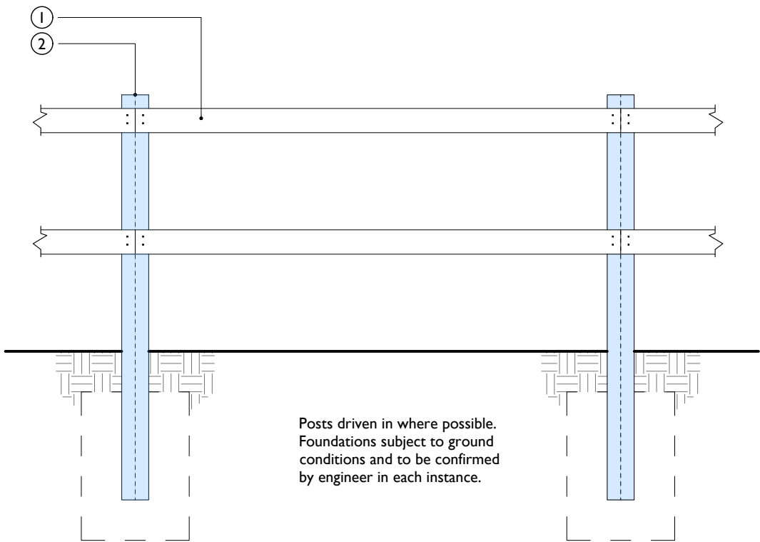
900mm Post and 2 rail fence 1:20
