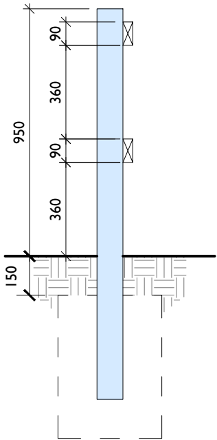
Section 1:20
