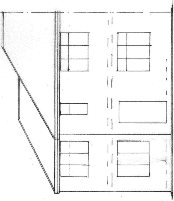
FRONT ELEVATION (BEFORE)
