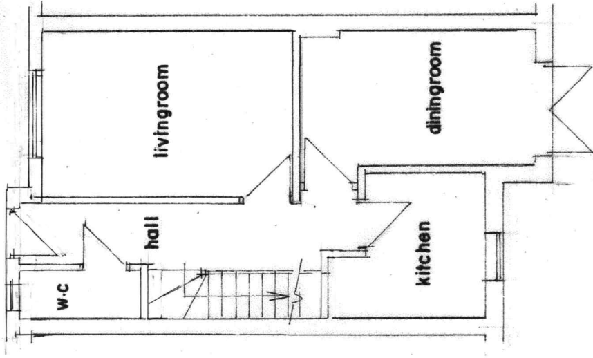
G.F. PLAN (EXISTING)
