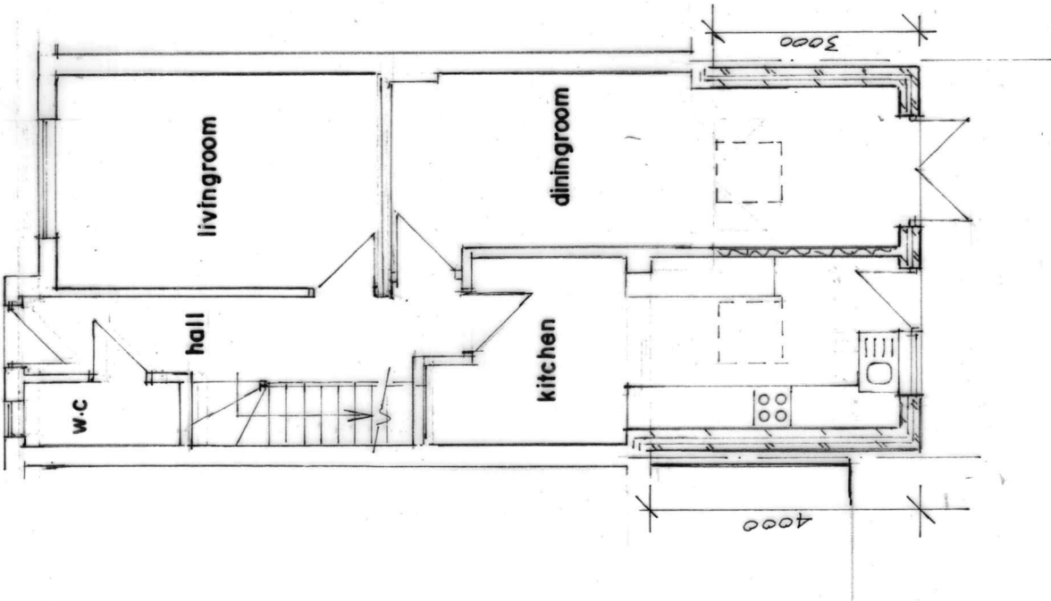
GROUND FLOOR PLAN (PROPOSED)
