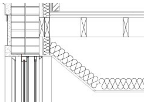
SUSPENDED CEILING DETAIL AT WINDOW
