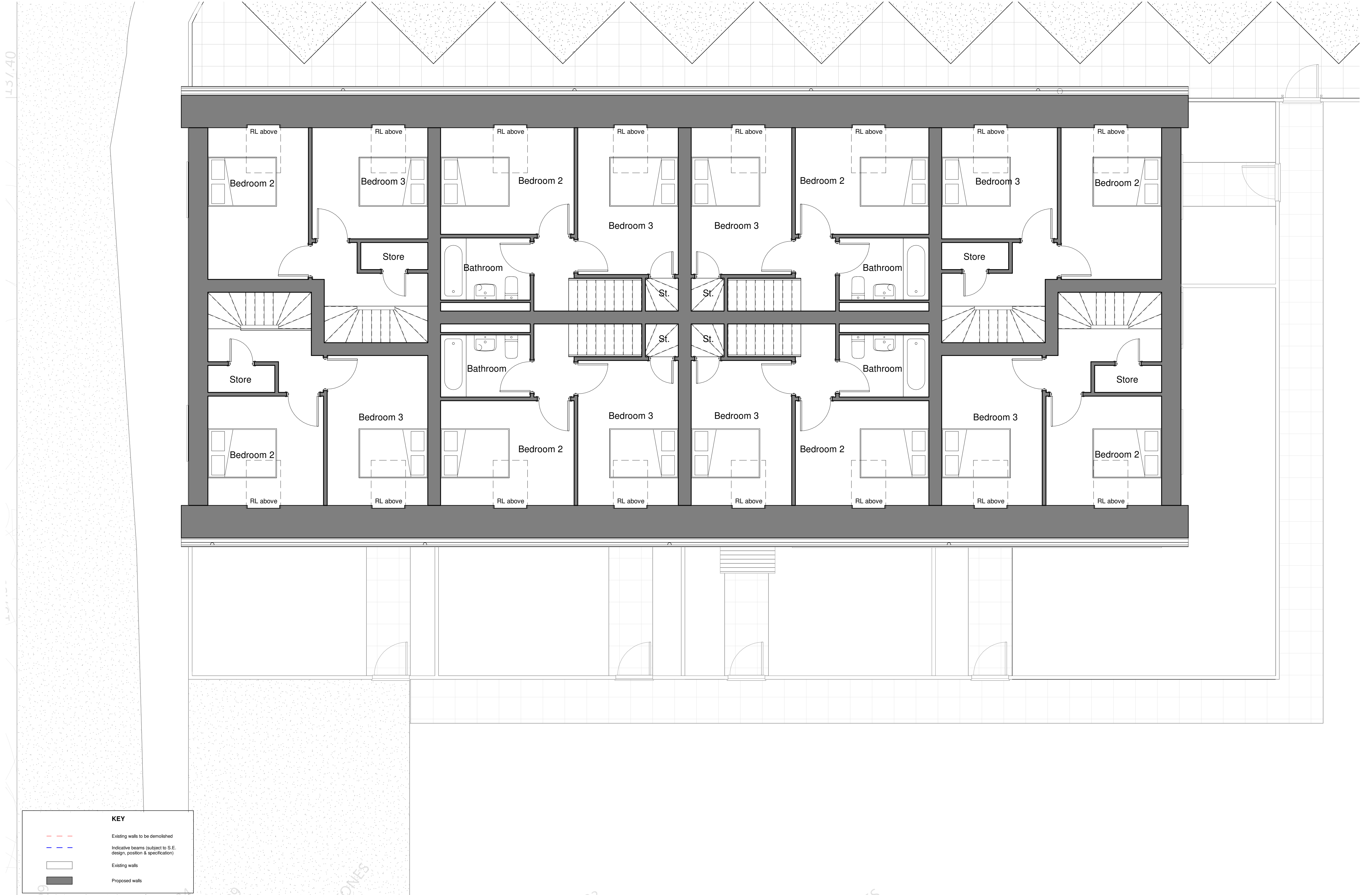
1 Proposed Level 2 1 : 50
