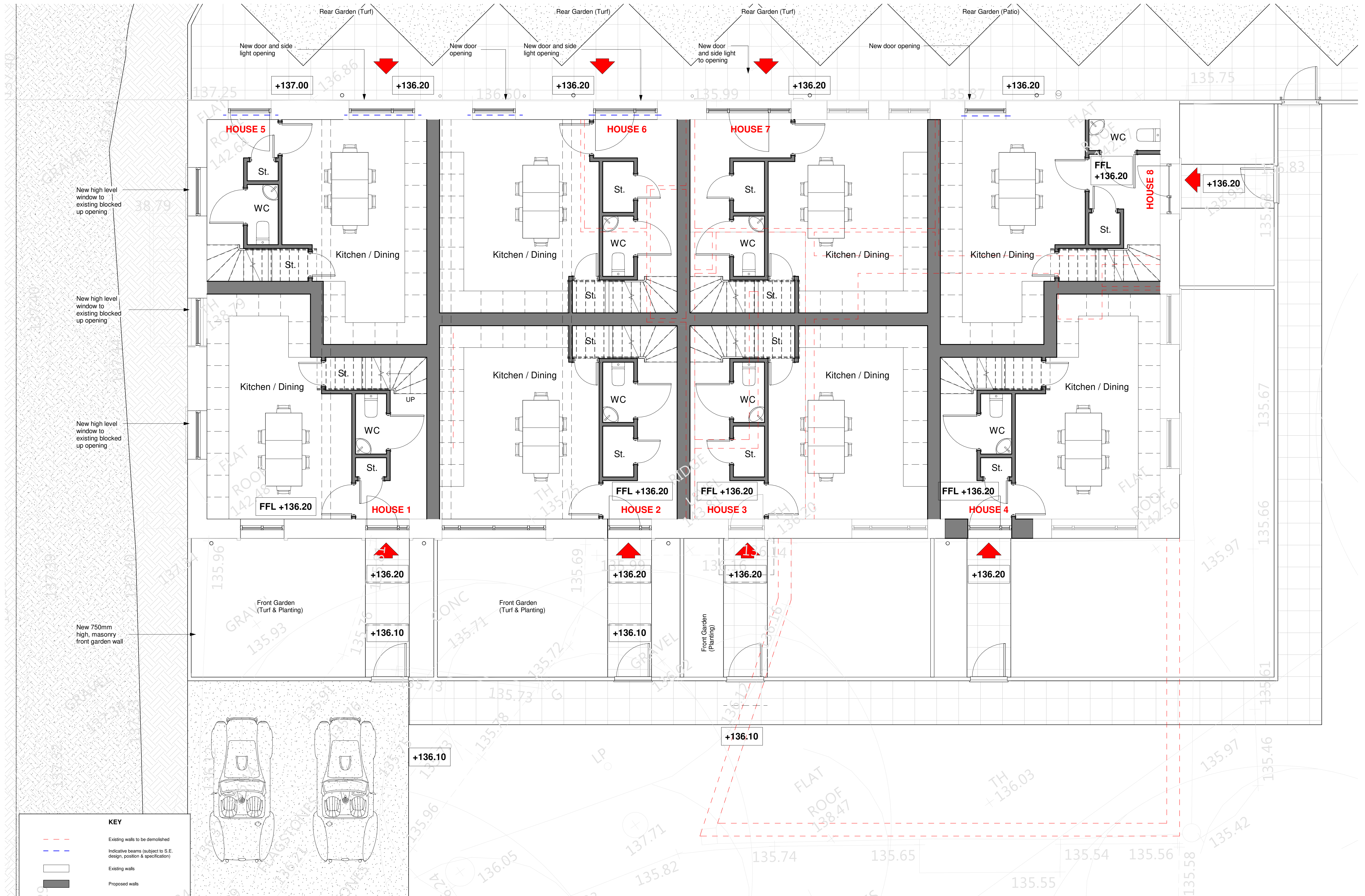
1 Proposed Level 0 1 : 50
