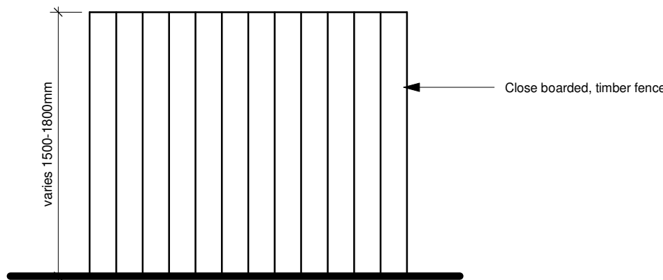
Timber Boundary / Enclosure Elevation
