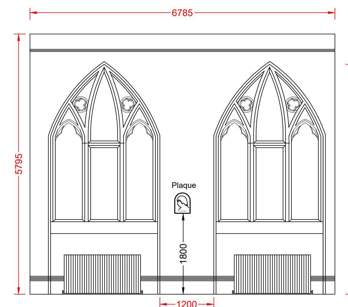
Elevation Of Proposed Location Of Memorial Plaque
