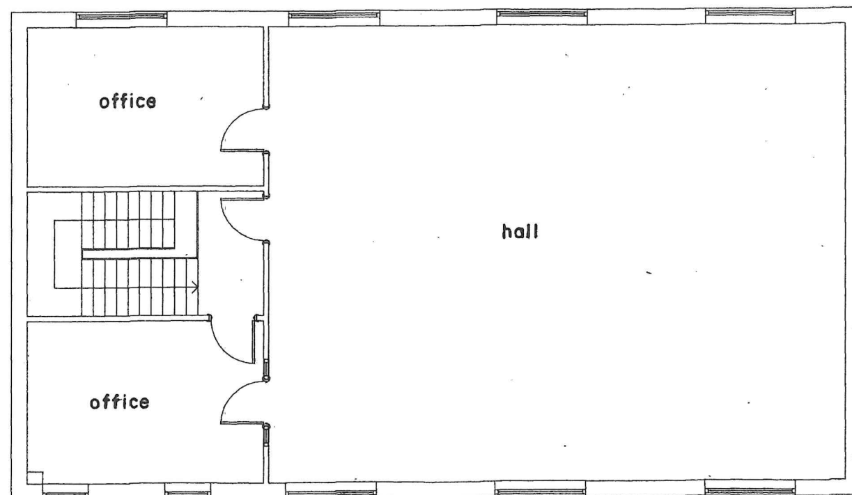
FIRST FLOOR PLAN SCALE 1:100 (EXISTING)
