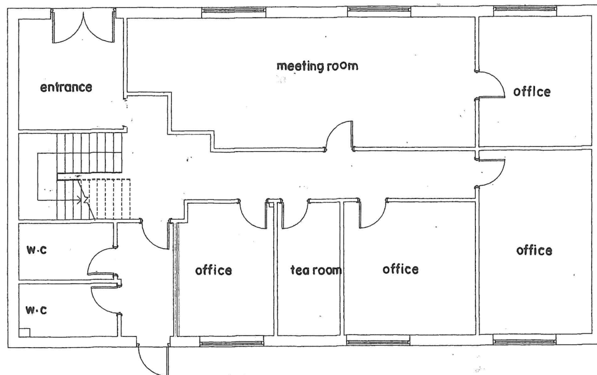
GROUND FLOOR PLAN SCALE 1:100 (EXISTING)
