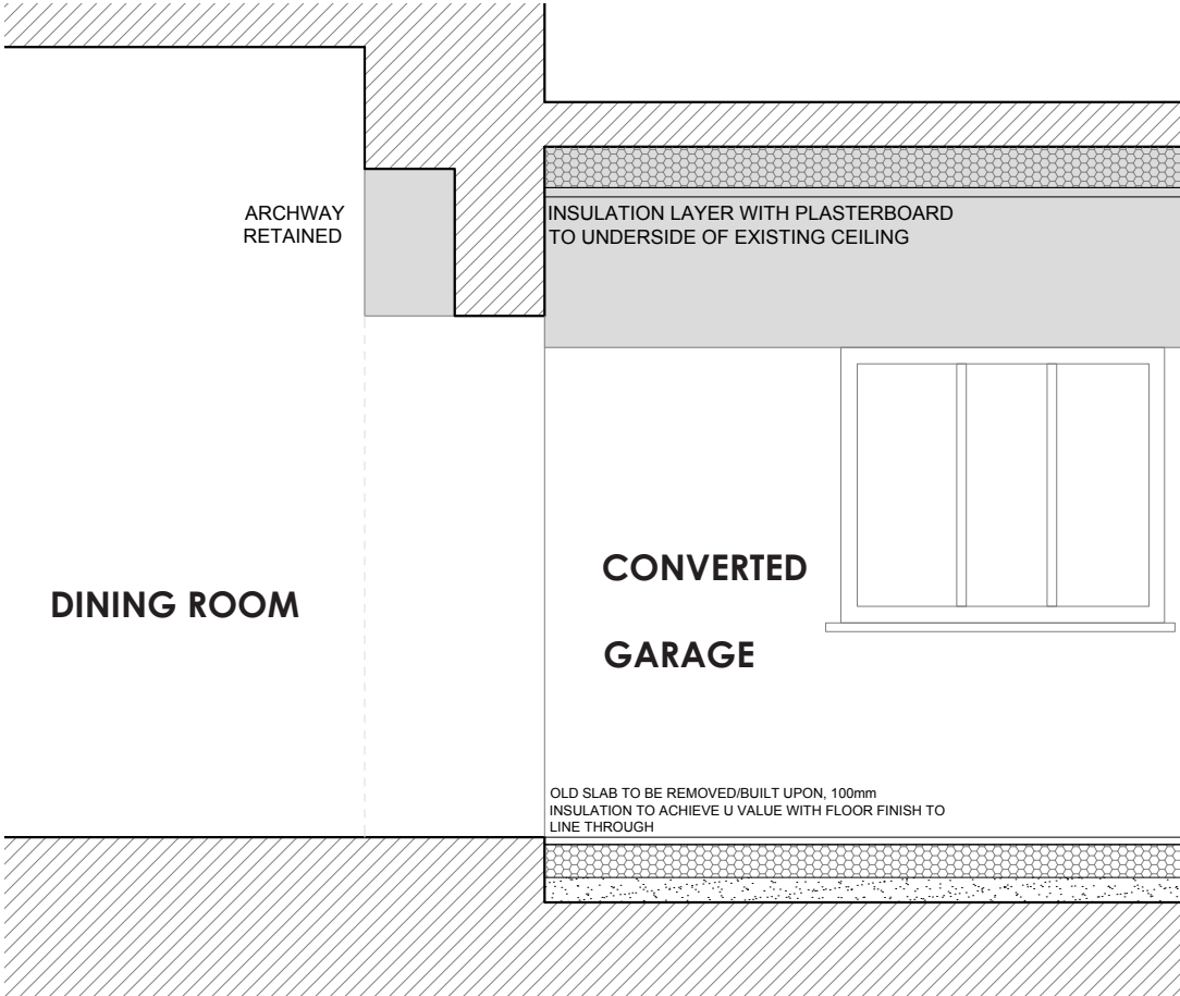
PROPOSED SECTION THROUGH ARCHED DUMMY DOOR 1:25 @ A3
