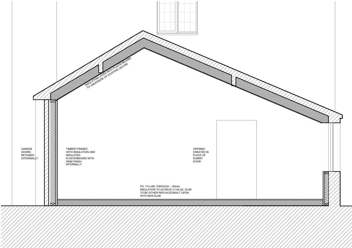
PROPOSED SECTION THROUGH GARAGE 1:50 @ A3
