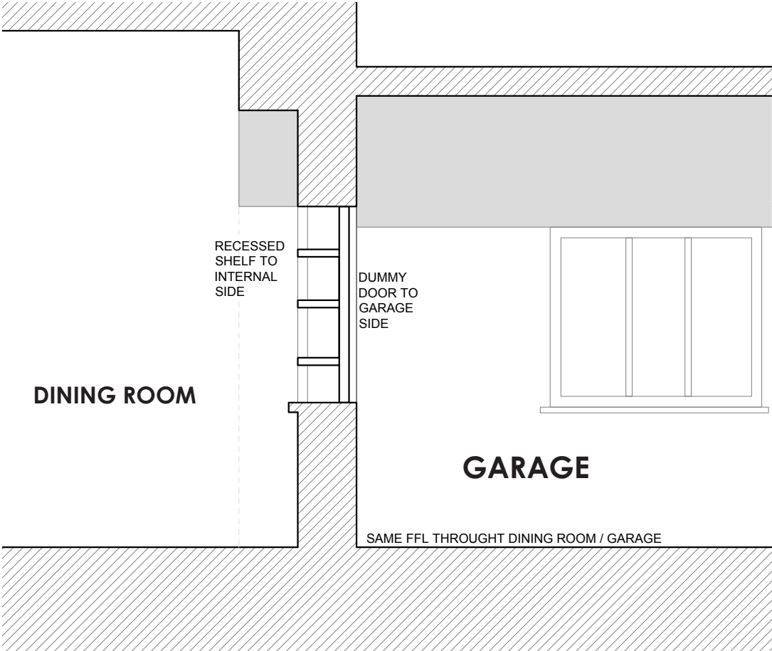
EXISTING SECTION THROUGH ARCHED DUMMY DOOR 1:25 @ A3
