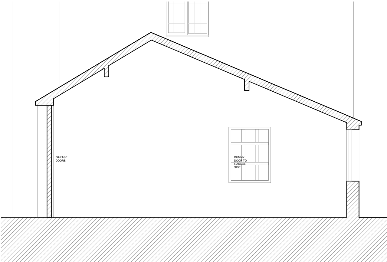
EXISTING SECTION THROUGH GARAGE 1:50 @ A3
