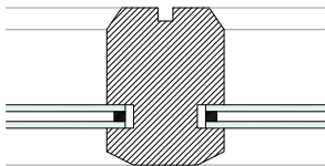
Vertical Mullion: Fixed Window
