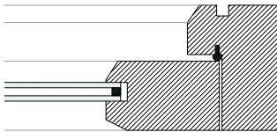
Jamb: Outward Opening Door
