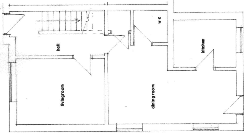
G.F. PLAN (EXISTING)
