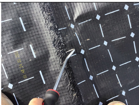
Testing the hand welded membrane lap joints
