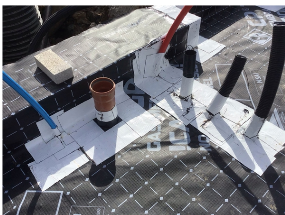
Pipe detailing
