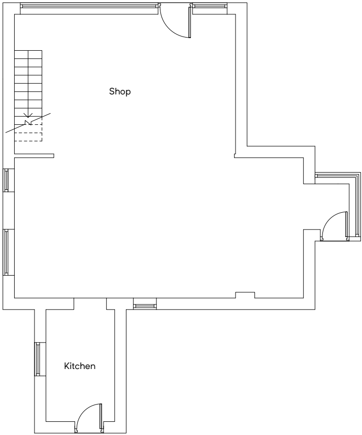
GROUND FLOOR PLAN (EXISTING)
