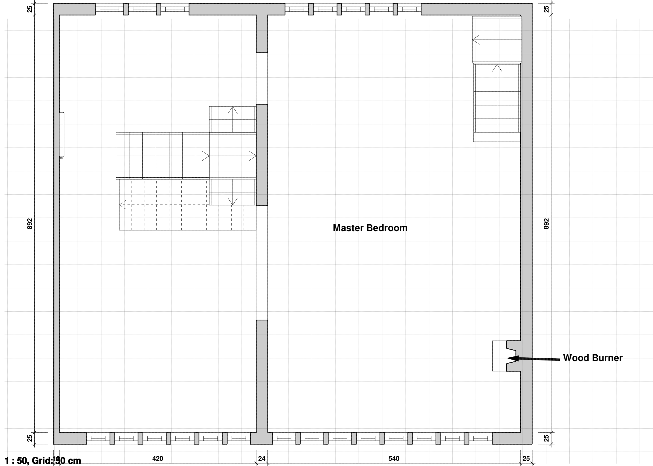
Existing 2nd Floor Plan
