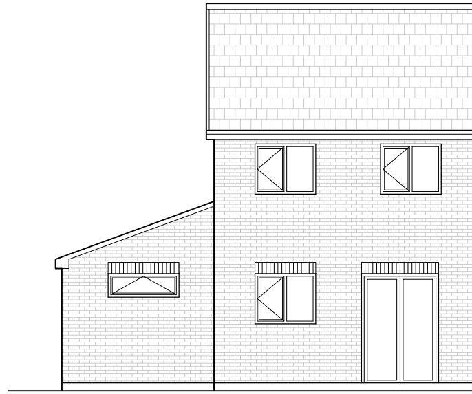
PROPOSED REAR ELEVATION 1:100 @ A3
