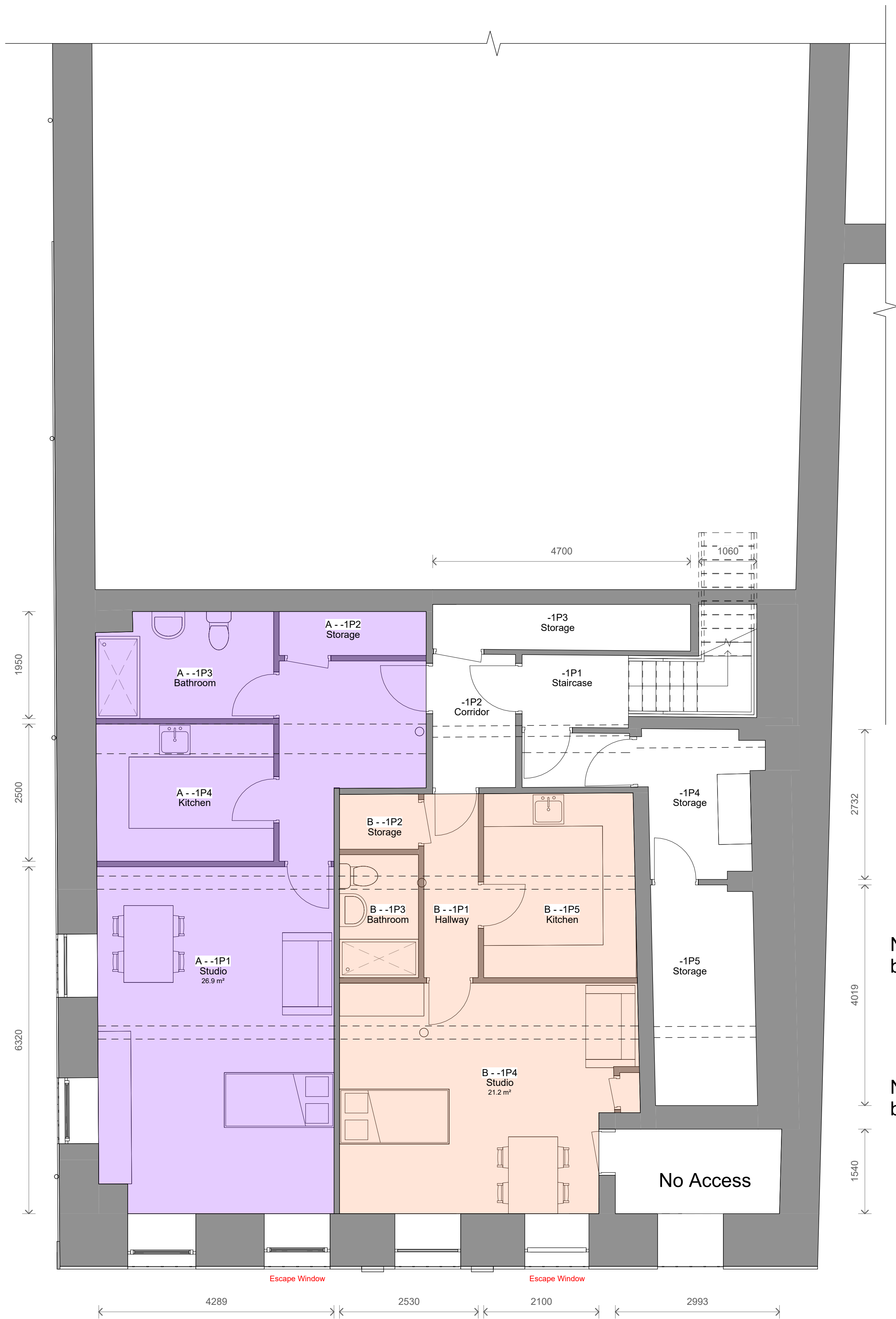
1 Level B1 - Proposed 1 : 50
