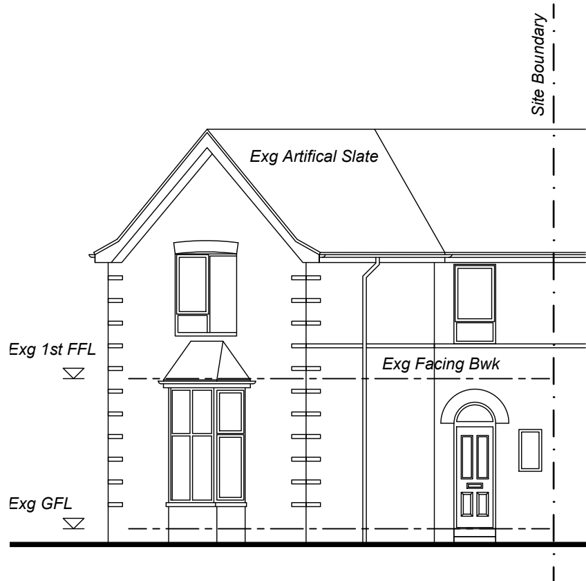
EXISTING FRONT ELEVATION (SOUTH)
