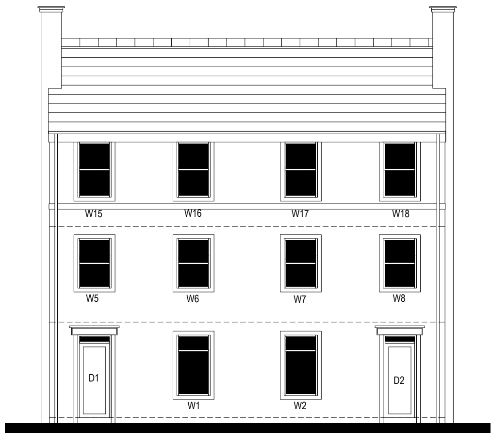
FRONT ELEVATION
