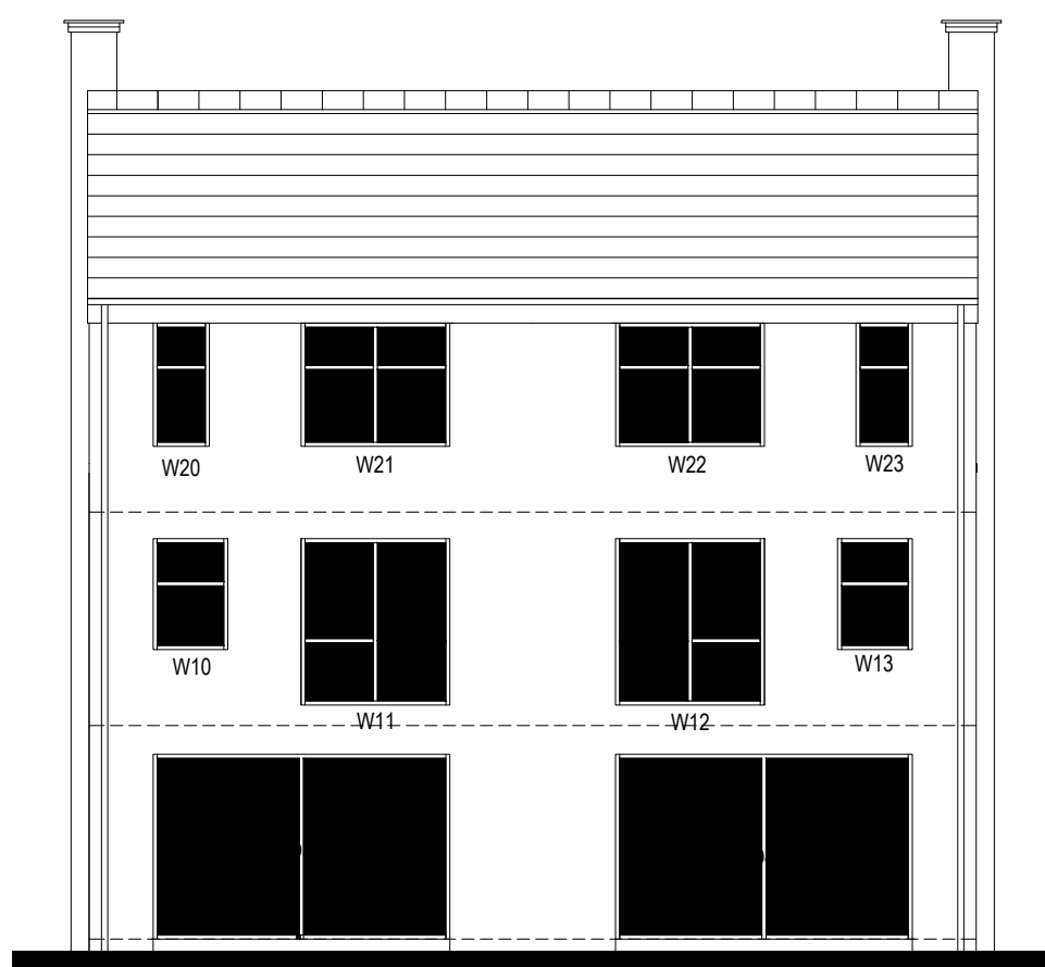
REAR ELEVATION
