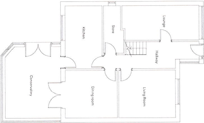
GROUND FLOOR PLAN (EXISTING)
