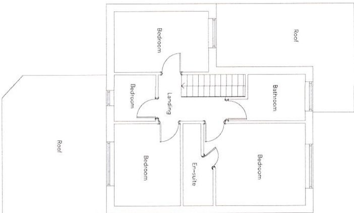
FIRST FLOOR PLAN (EXISTING)
