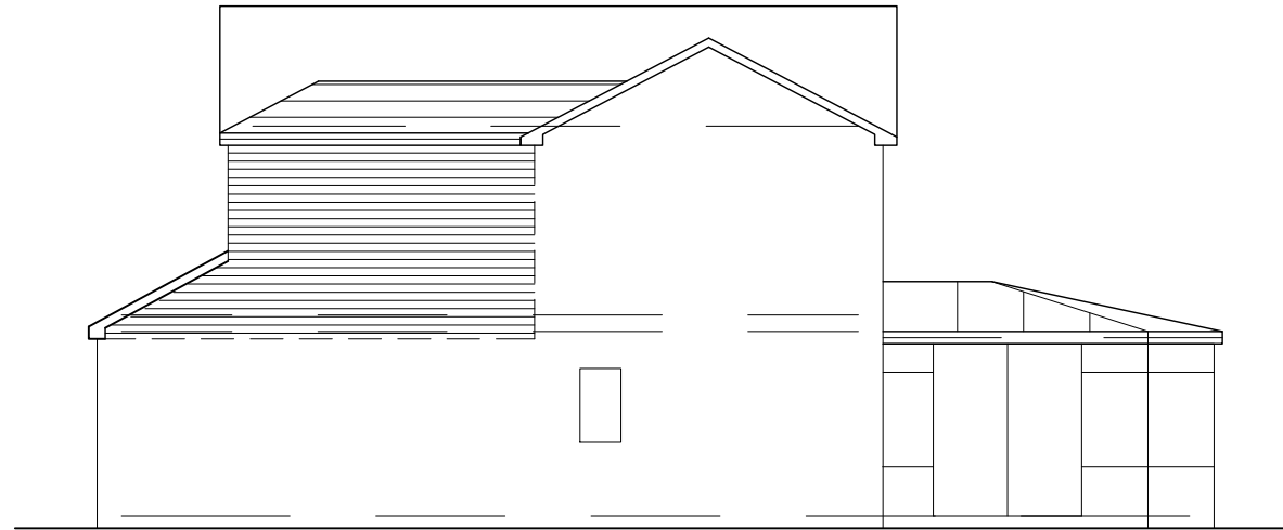
SIDE ELEVATION (PROPOSED)
