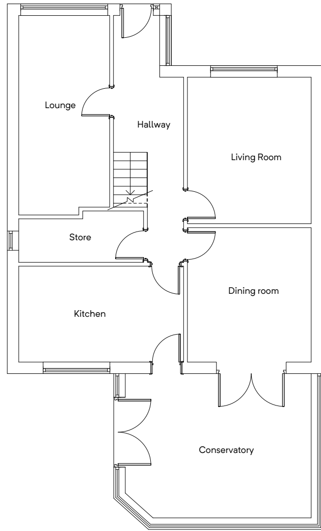
GROUND FLOOR PLAN (PROPOSED)
