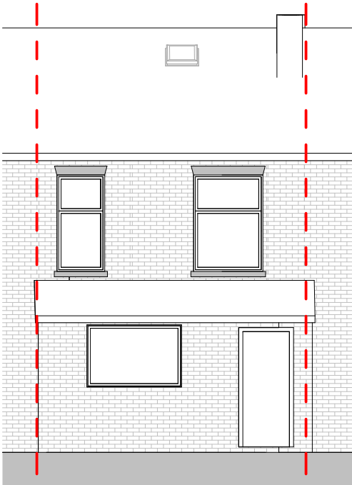
Rear Elevation as Existing
