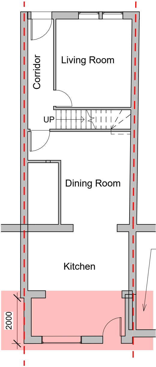
Ground Floor - Previous Application 1 : 100
