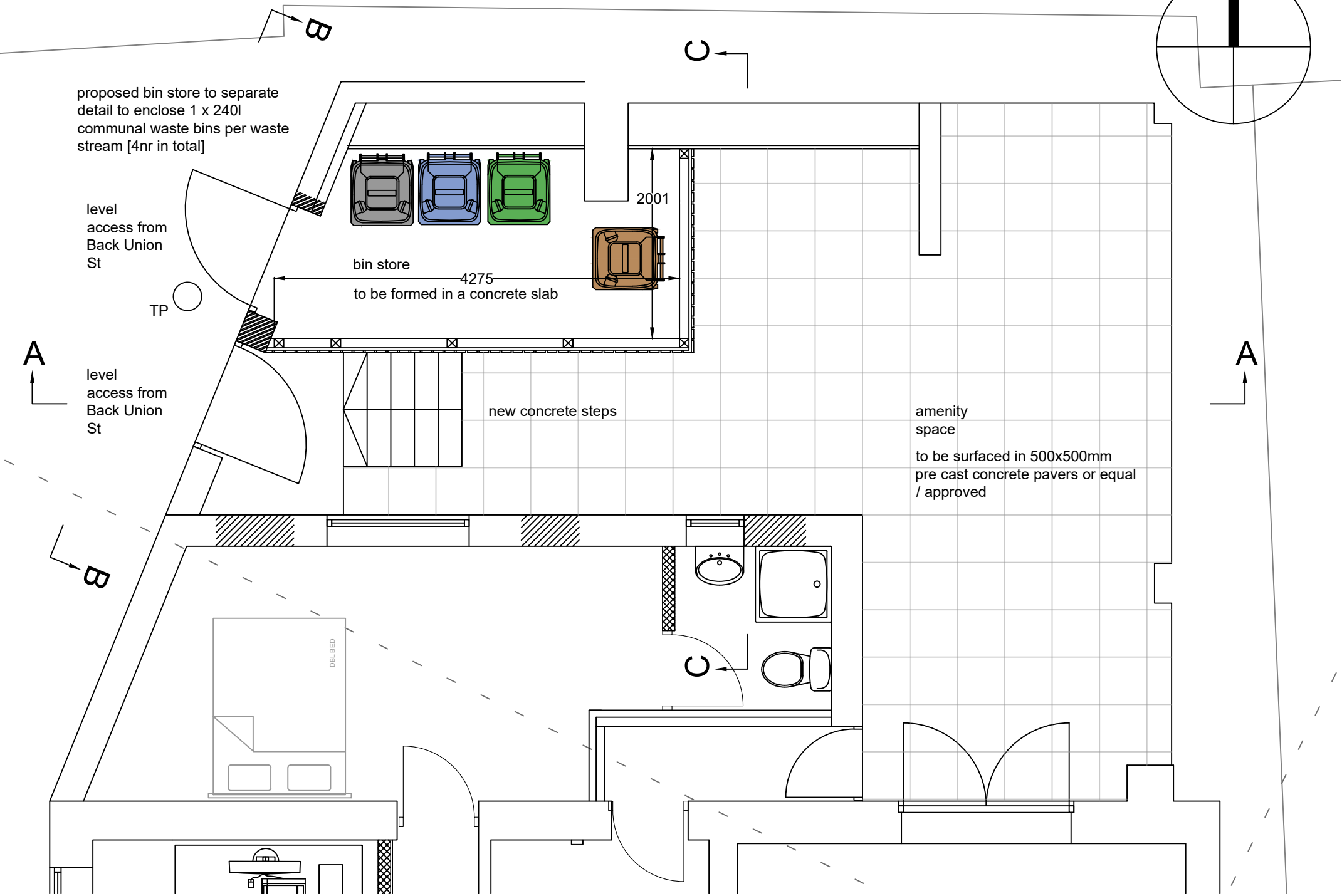
proposed yard / binstore plan scale 1 - 50
