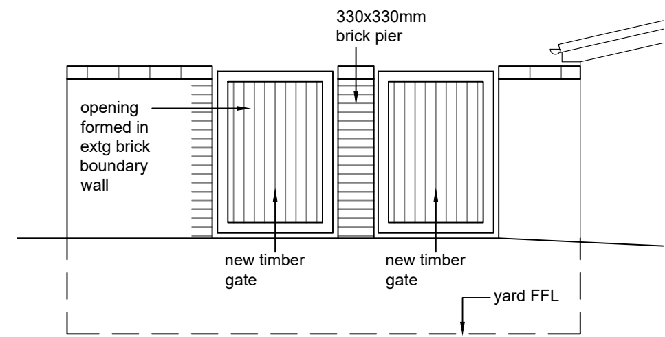
proposed elevation BB scale 1 - 50
