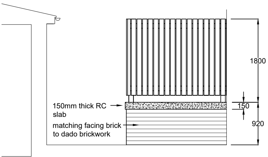
proposed elevation CC scale 1 - 50
