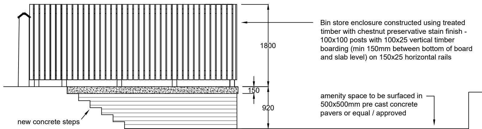
proposed elevation CC scale 1 - 50
