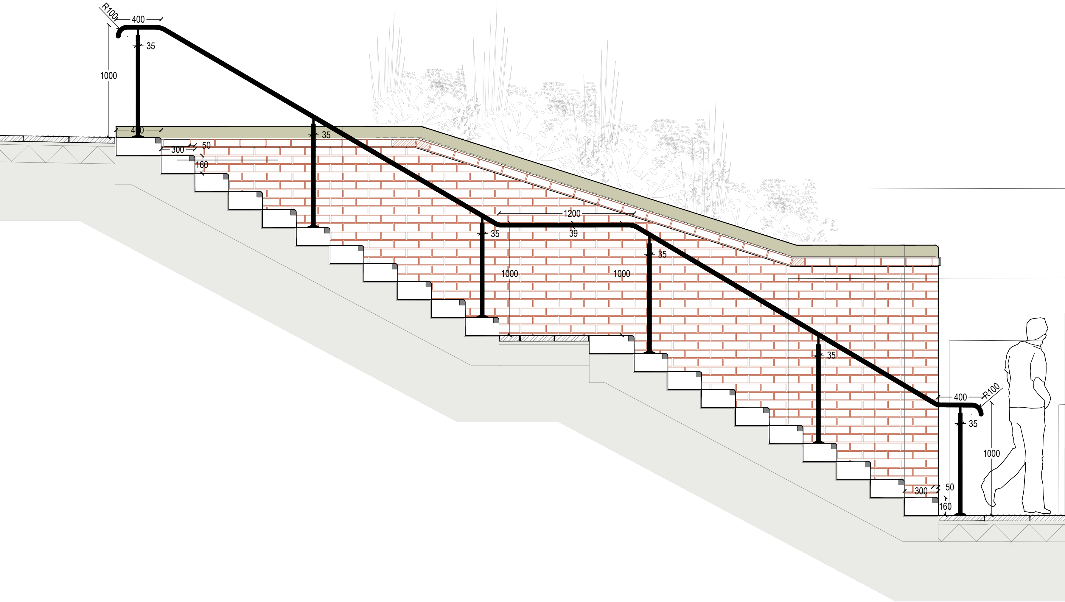
02 ST1 Sandstone Steps Section A-A (Basement Access) Scale 1: 20 @A1
