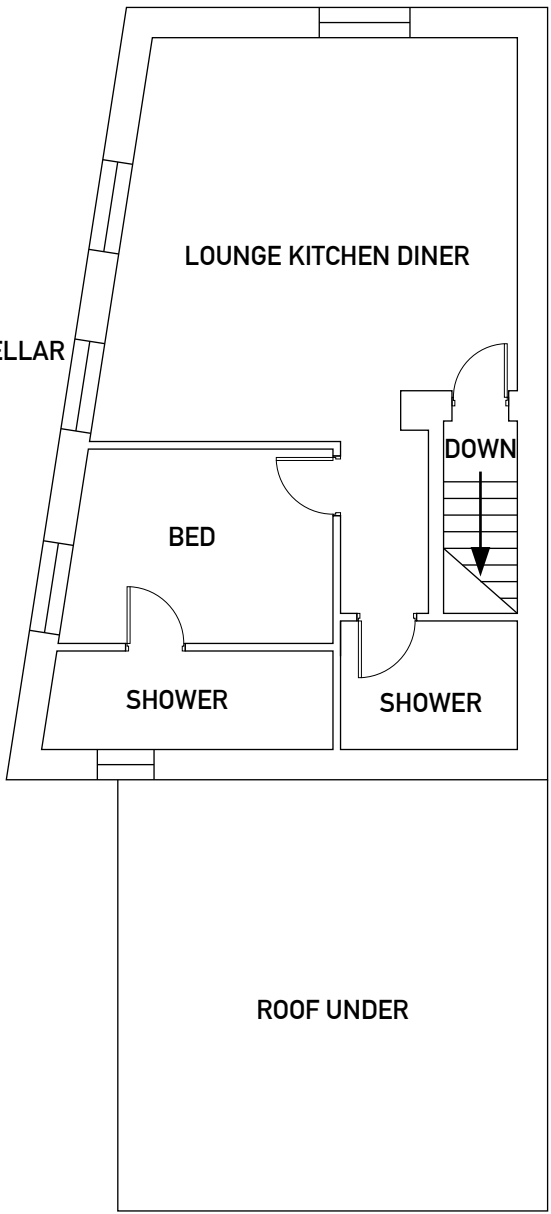
EXISTING 1ST FLOOR PLAN
