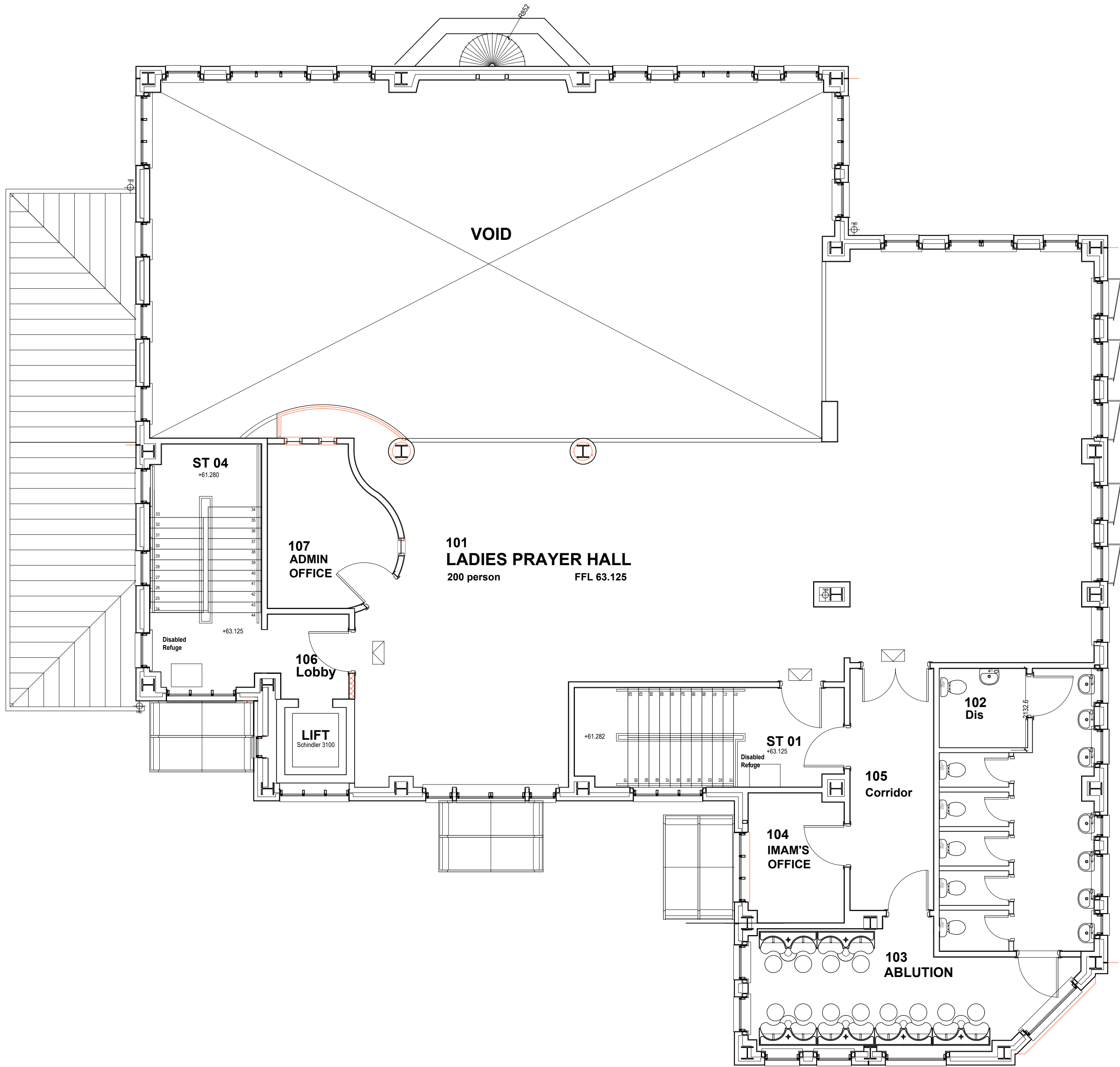
EXISTING FIRST SCALE 1 : 75
