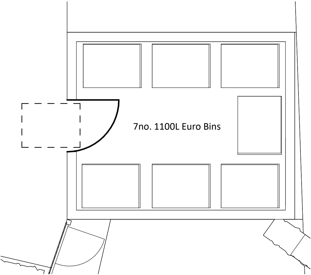
Proposed Bin Store Plan 1 : 50
