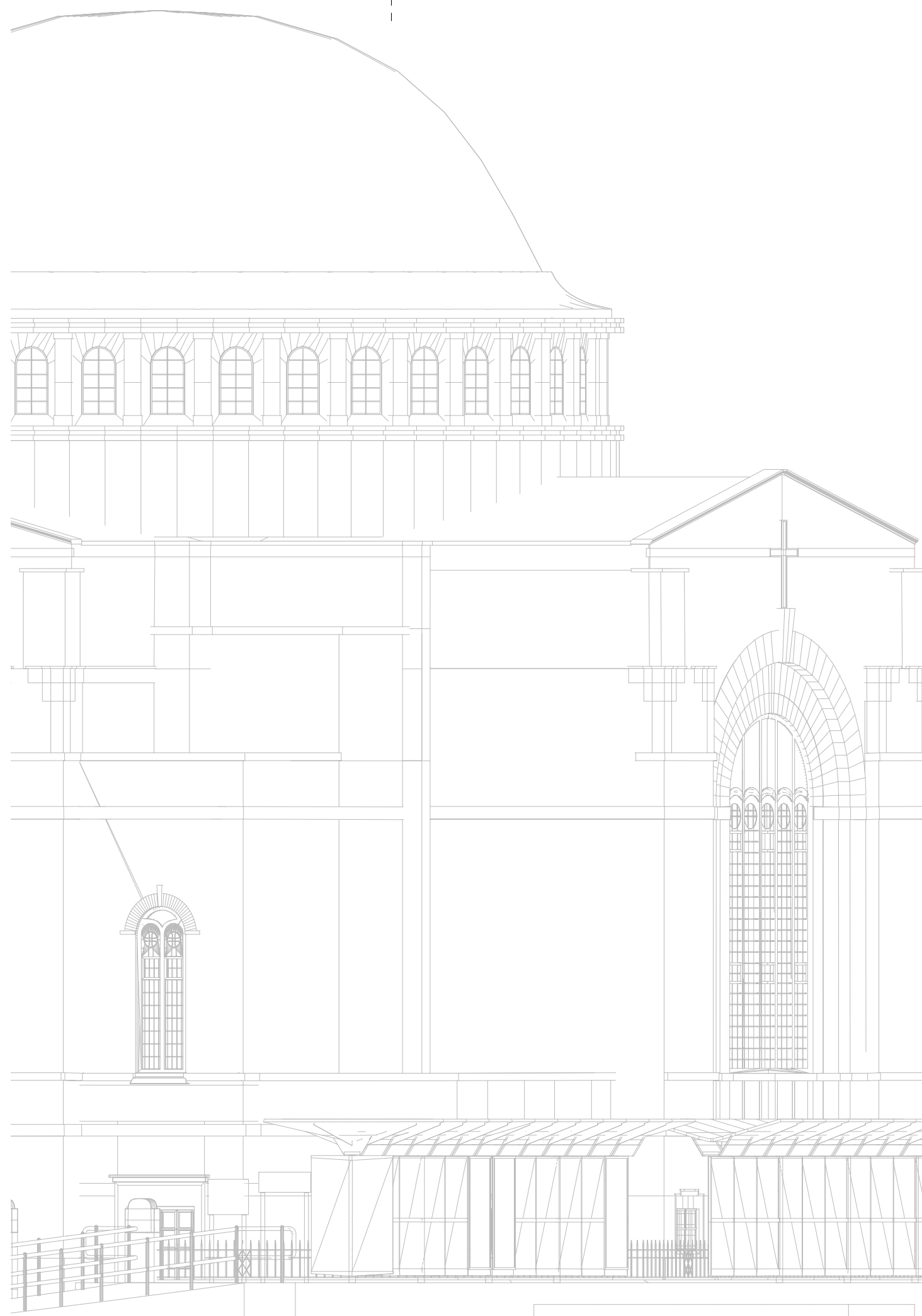
ELEVATION 1-1
