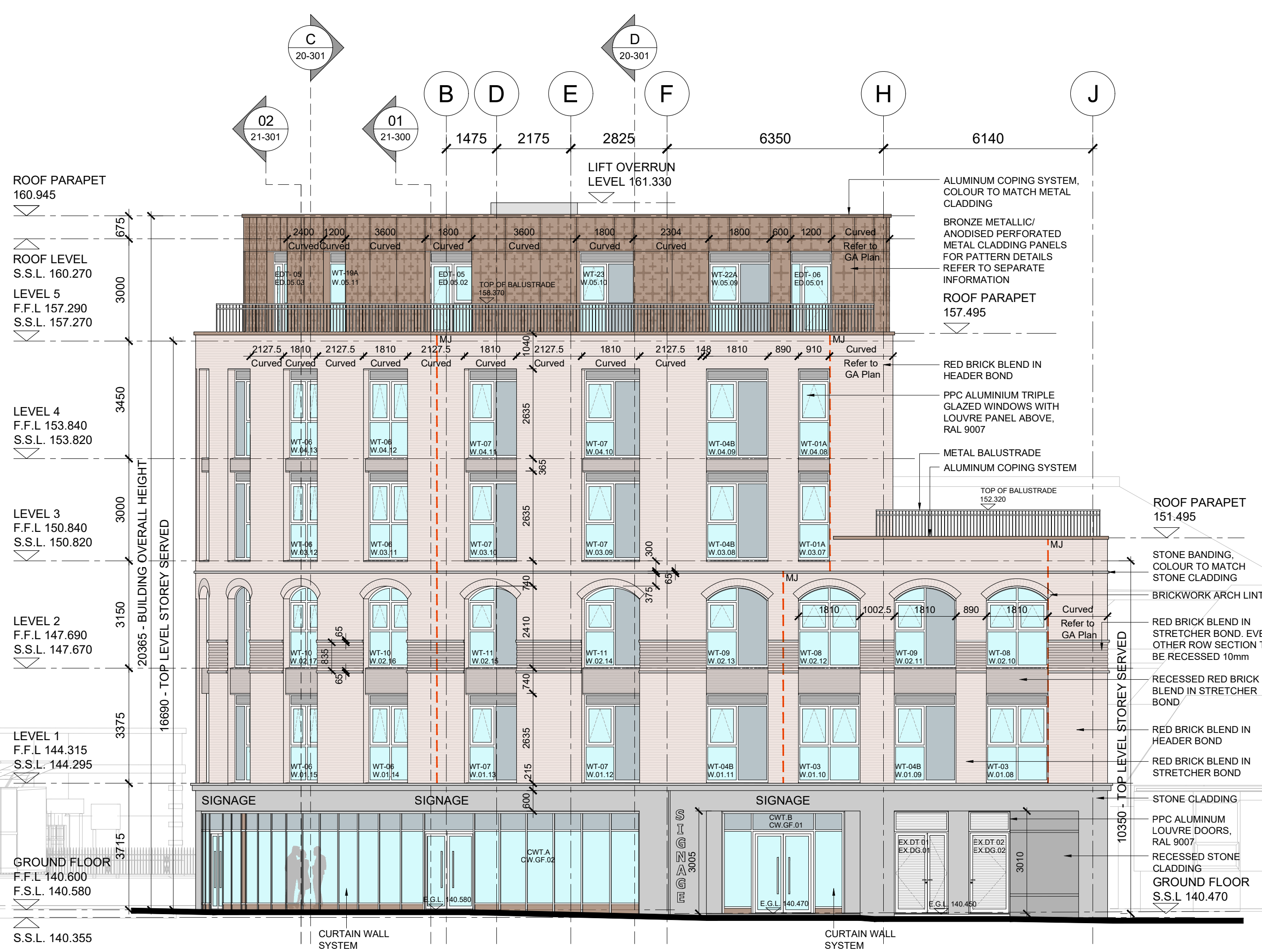
ELEVATION 2-2
