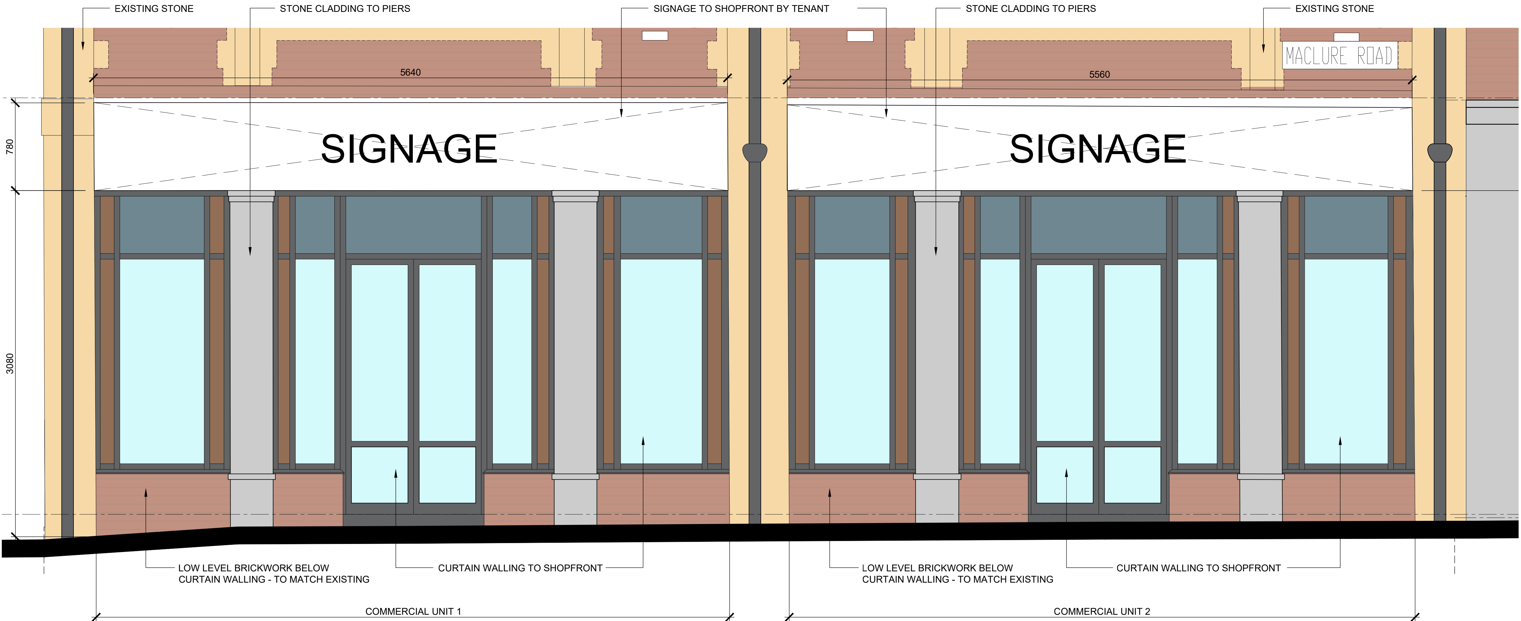
ELEVATION 01. 1:20 SCALE
