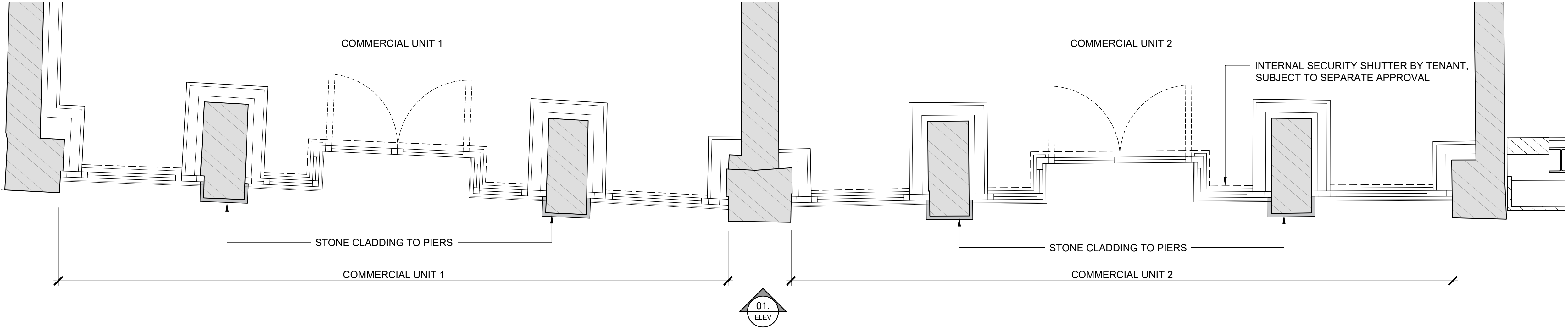
PLAN 1:20 SCALE
