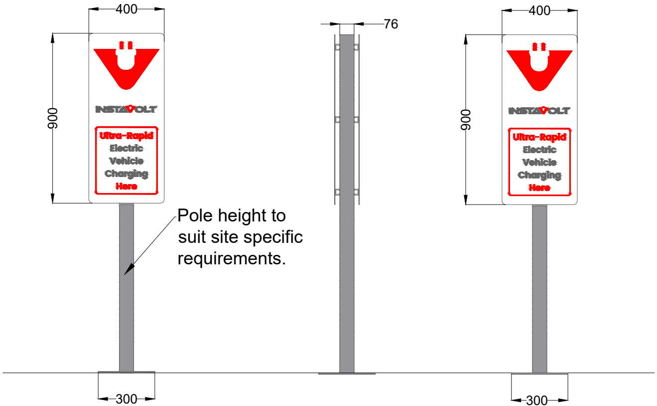
A Totem - Front View
