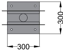
D Totem - Plan View
