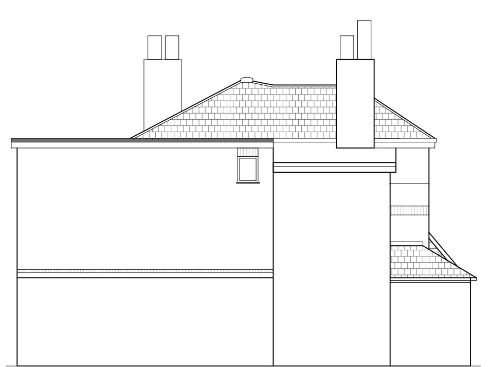
Existing Side Elevation(West) Scale - 1:100@A3
