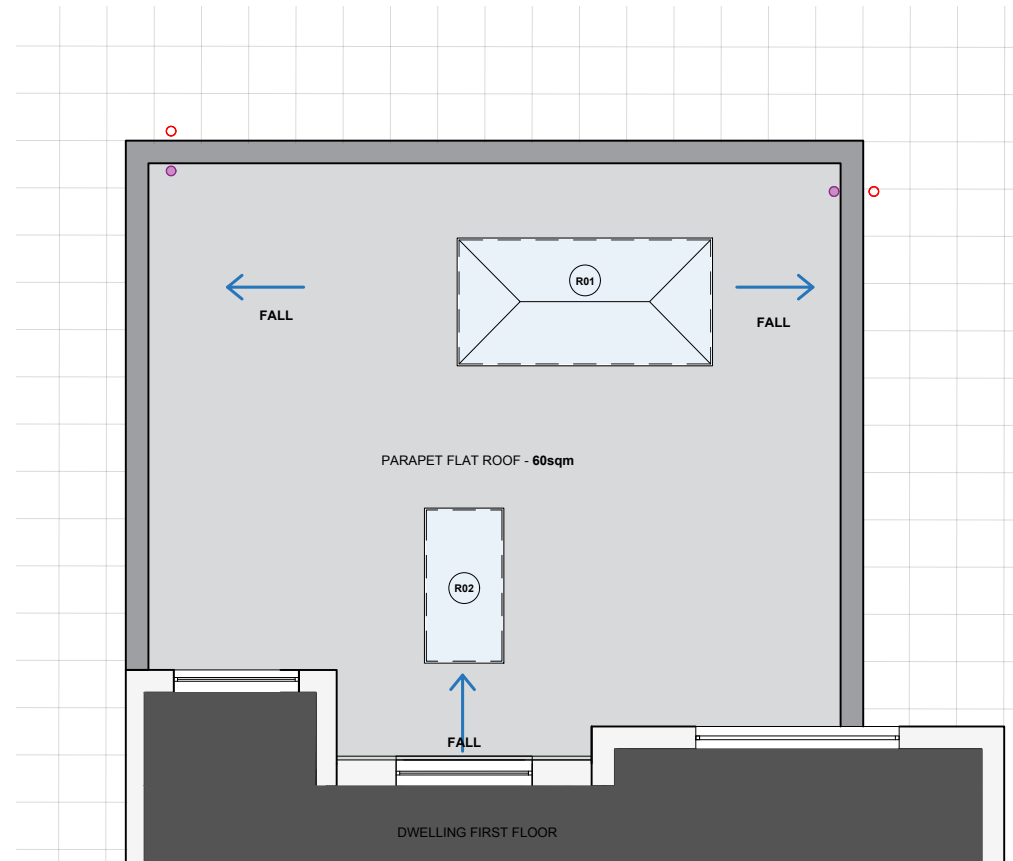
Scale - 1:100@A3
