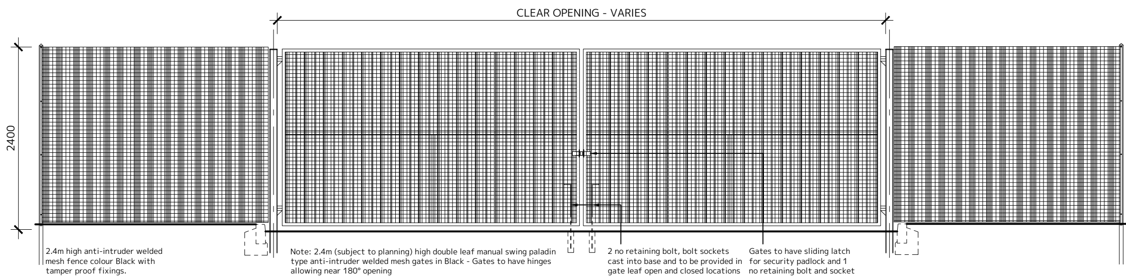
Weldmesh Fence, Vehicle Gate 1:50
