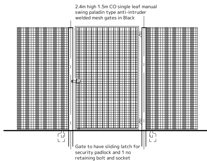
Weldmesh Fence, Pedestrian Gate 1:50
